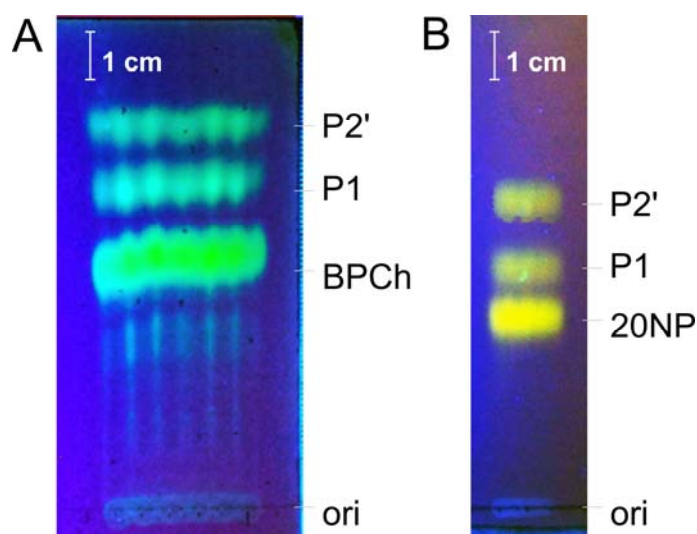
Fig. 2. A photo of TLC plate, showing separation of the P1-type and P2'-type products formed during incubation of BPCh (A) and 20NP (B) (25 \mu M both) with \text{NAD}^+ (1 mM) and cholesterol dehydrogenase ( 3\beta -HSD) from Nocardia sp. (0.35 U/ml). P1 and P2' designate the 4-en-3-one and 5-ene-3-one derivatives of the fluorescent substrate, respectively.
